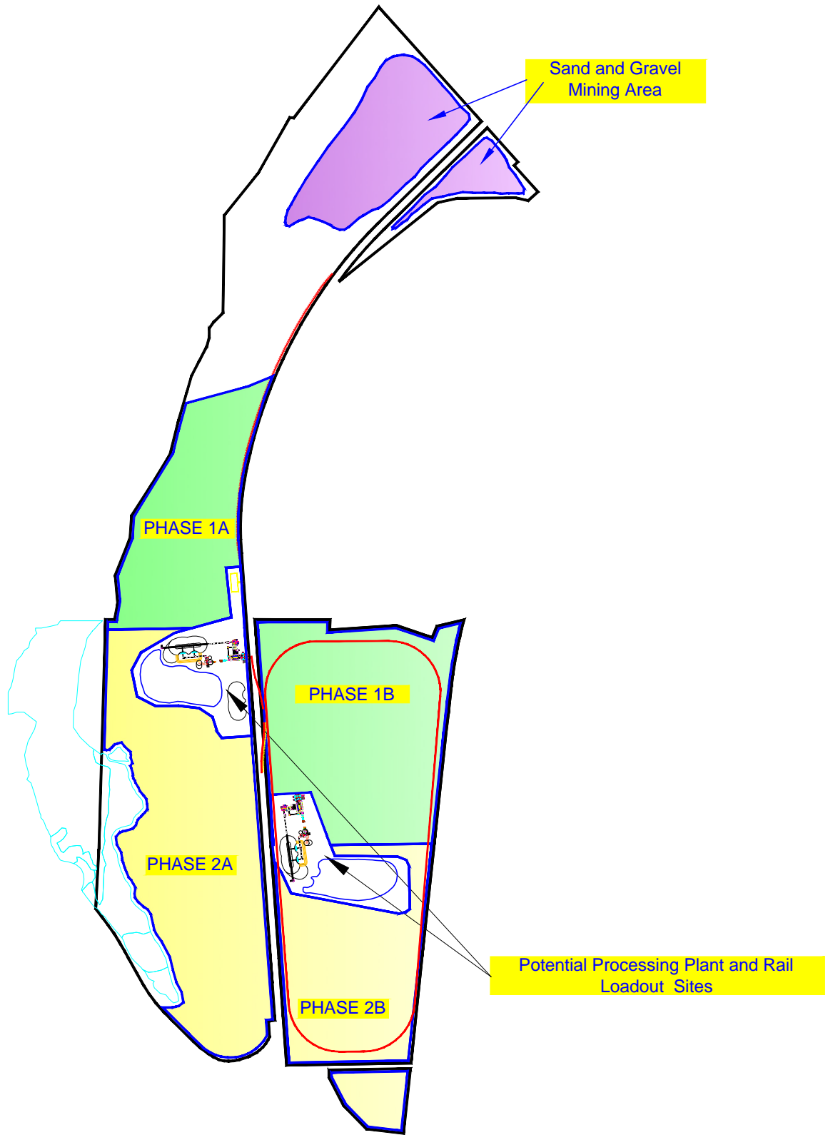
Figure 5-2: Alternative 2 1.2 MT/YR BRP and MS-S Concept Mine Plan Merriam Junction Sands Scoping EAW
