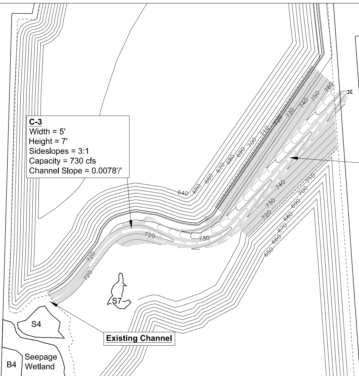
Figure 3.4.4 Channel Design - Malkerson Sales Merriam Junction Sands DEIS
