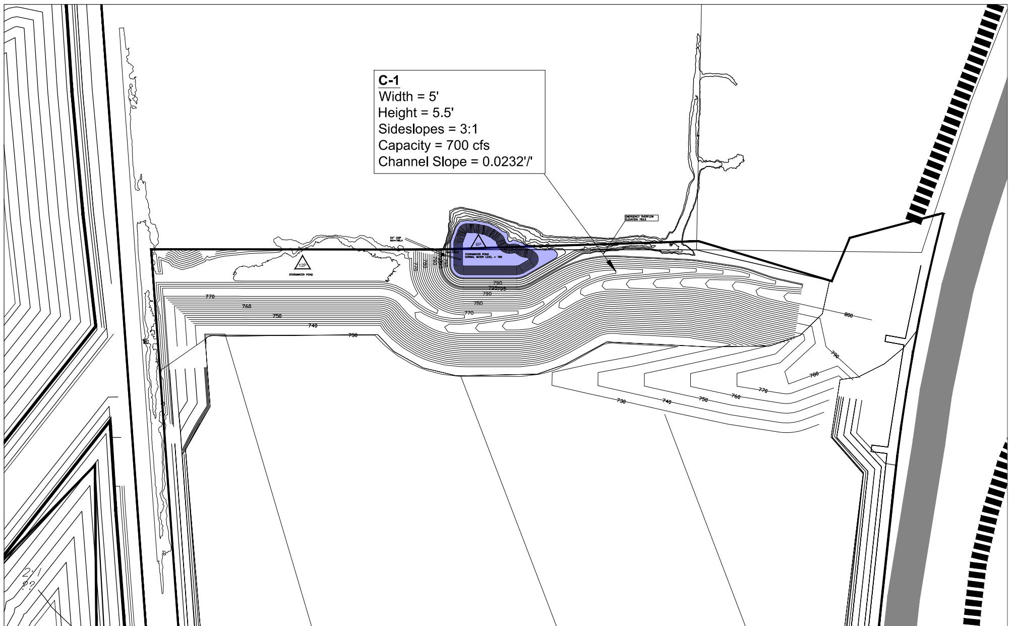
Figure 3.4.3 Channel Design - Bryan Rock Merriam Junction Sands DEIS
